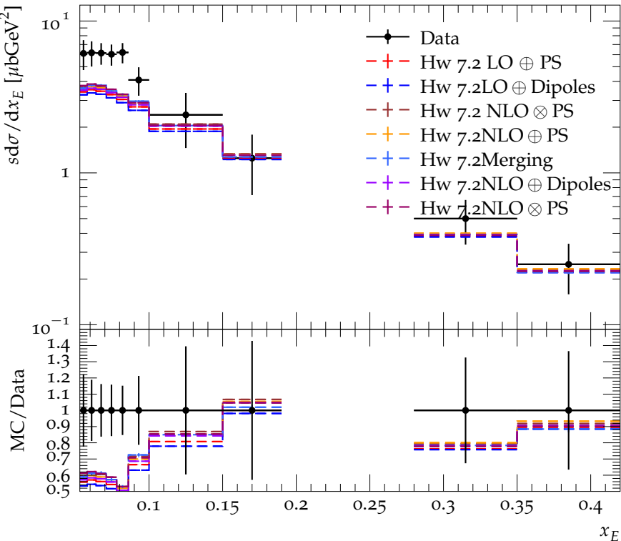
K^\pm spectrum for E_{\text{CMS}} = 22 GeV
