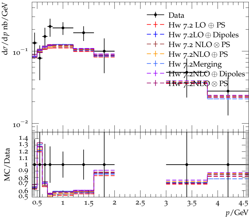
p, \bar{p} spectrum for E_{\text{CMS}} = 22 GeV
