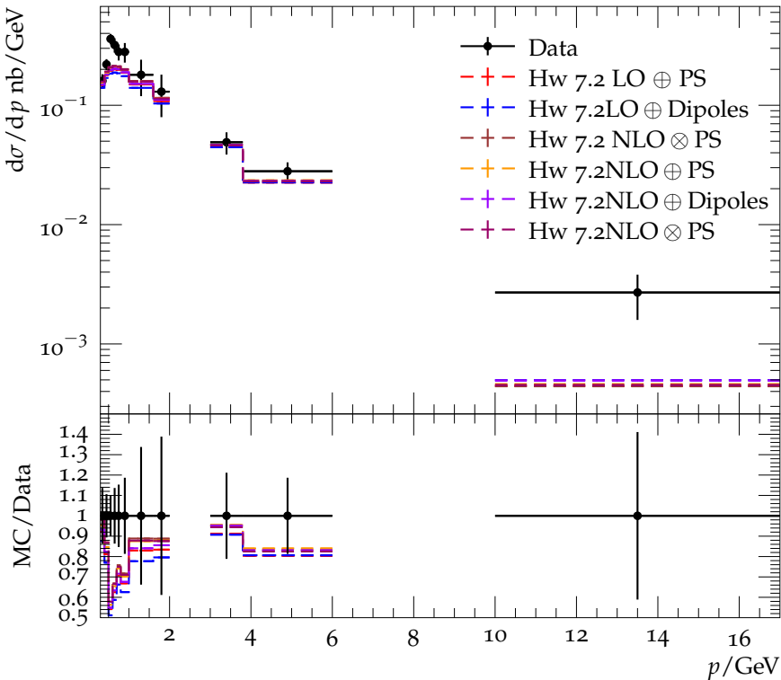
K^\pm spectrum for E_{\text{CMS}} = 34 GeV
