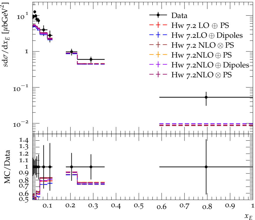
p, \bar{p} spectrum for E_{\text{CMS}} = 22 GeV
