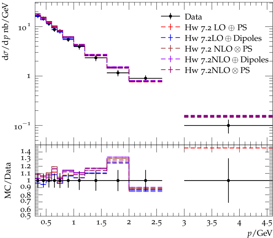
\pi^\pm spectrum for E_{\text{CMS}} = 14 GeV
