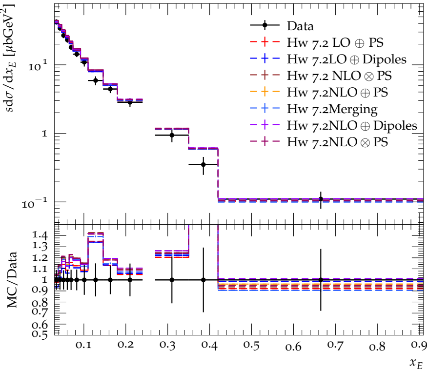
K^\pm spectrum for E_{\text{CMS}} = 14 GeV
