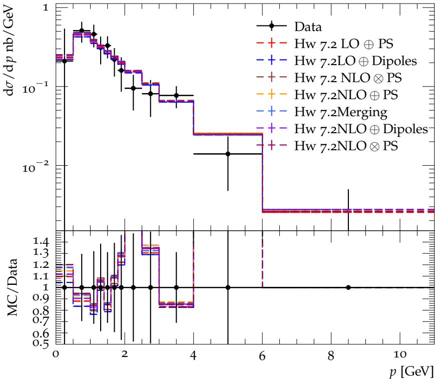
K^0, \bar{K}^0 momentum spectrum for E_{\text{CMS}} = 22 GeV
