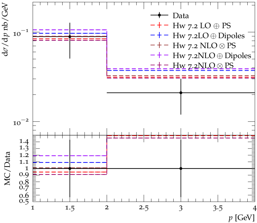
\Lambda^0, \bar{\Lambda}^0 momentum spectrum for E_{\text{CMS}} = 14 GeV
