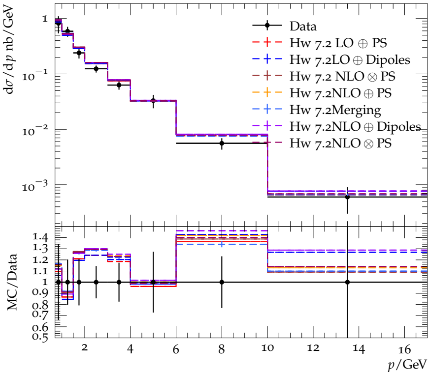
\pi^0 momentum spectrum for E_{\text{CMS}} = 34 GeV
