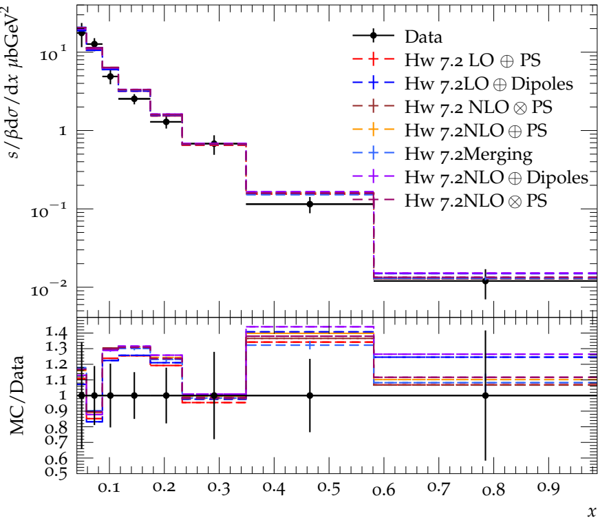
\pi^0 scaled momentum spectrum for E_{\text{CMS}} = 34 \text{ GeV}
