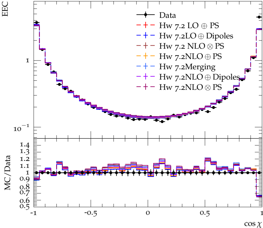
Energy-energy correlation, EEC for E_{\text{CMS}} = 22 \text{ GeV}
