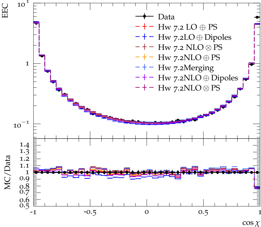
Energy-energy correlation, EEC for E_{\text{CMS}} = 43.5 GeV
