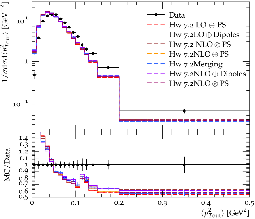
\langle p_{T\text{out}}^2 \rangle of charged particles w.r.t. sphericity axis at 35 GeV
