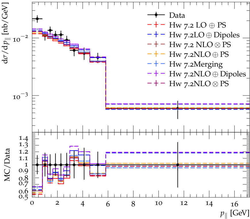
Momentum parallel to sphericity axis for \Lambda^0, \bar{\Lambda}^0 at 34.8 GeV
