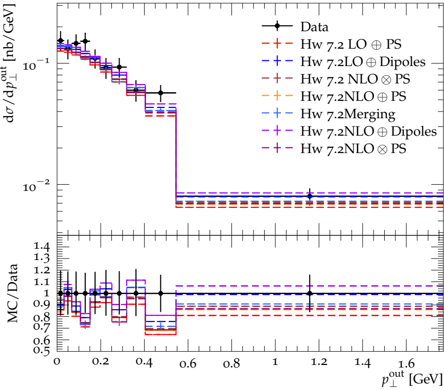
Out-plane momentum \perp to sphericity axis for \Lambda^0, \bar{\Lambda}^0 at 34.8 GeV
