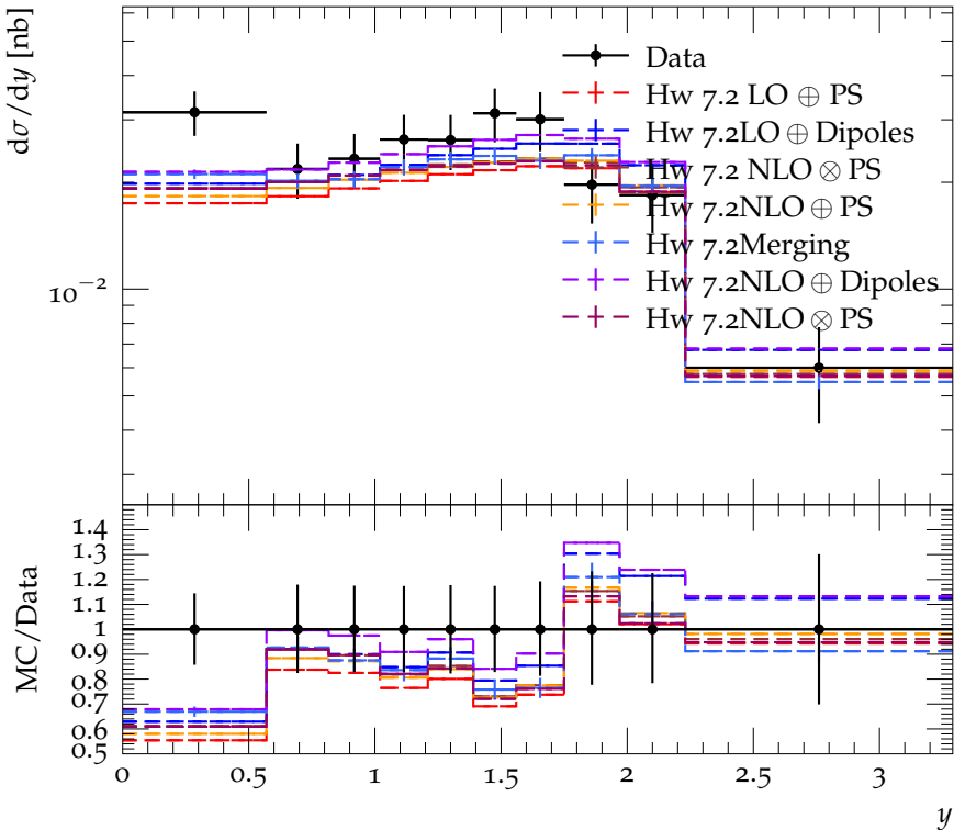
Rapidity w.r.t to sphericity axis for \Lambda^0, \bar{\Lambda}^0 at 34.8 GeV
