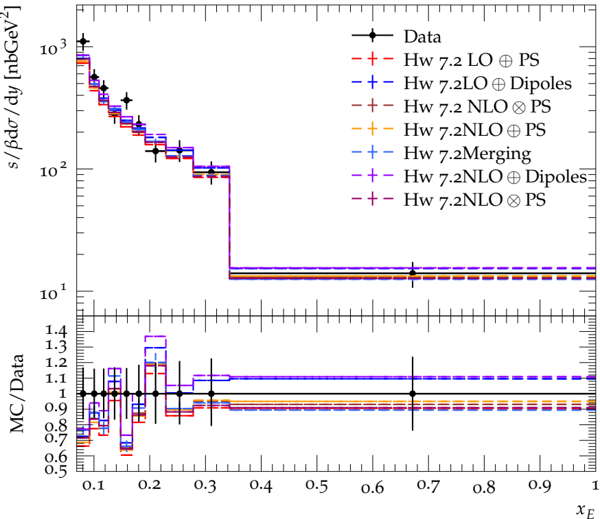
Scaled energy for \Lambda^0, \bar{\Lambda}^0 at 34.8 GeV
