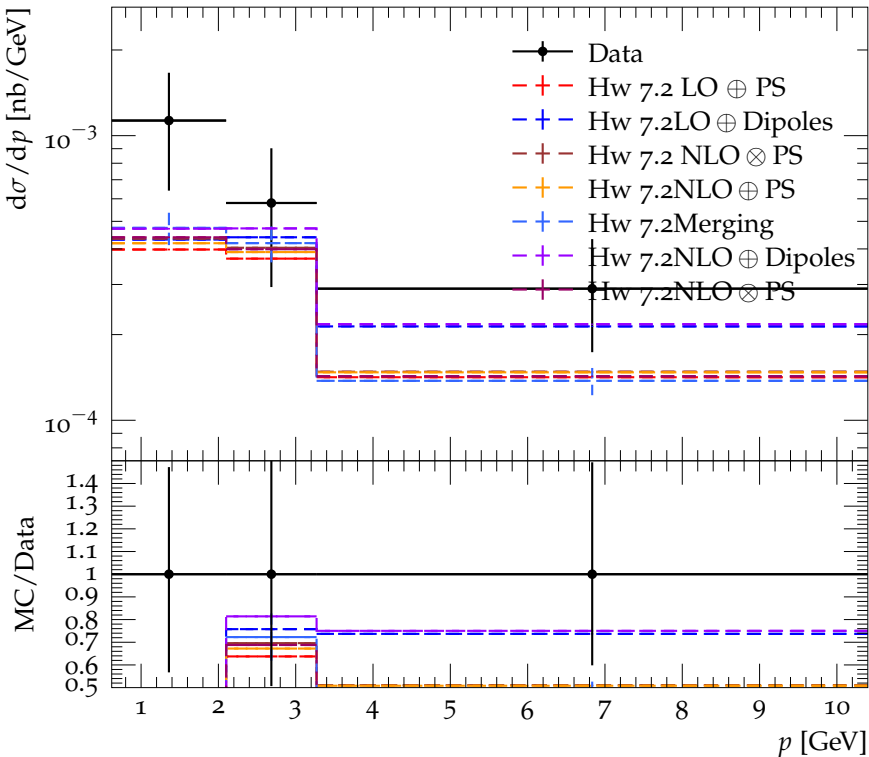
Momentum Spectrum for \Xi^- , \bar{\Xi}^+ at 34.8 GeV
