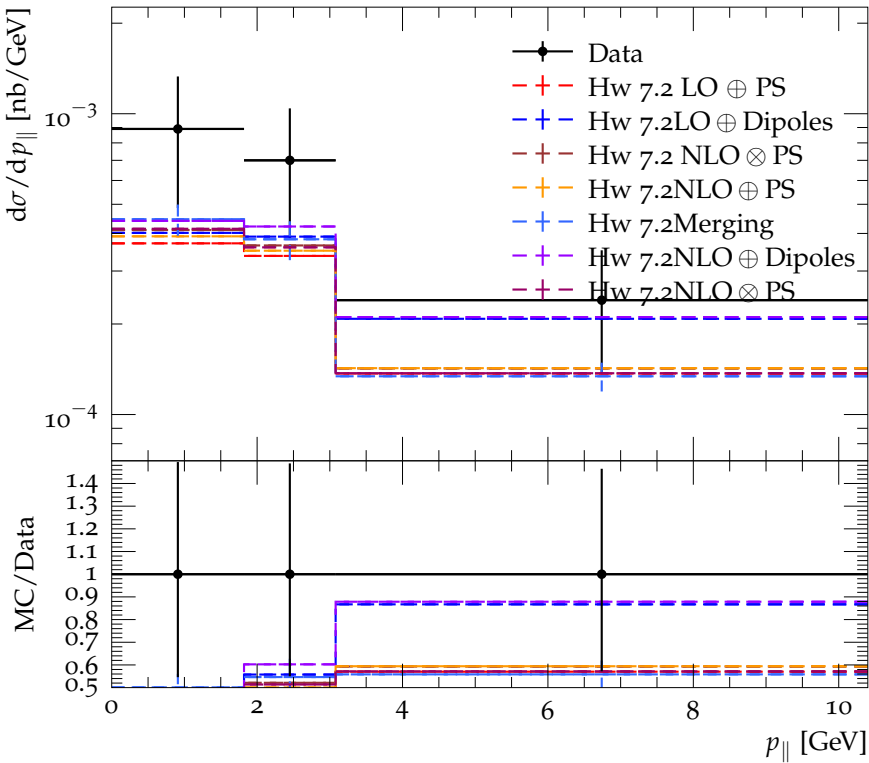
Momentum parallel to sphericity axis for \Xi^- , \bar{\Xi}^+ at 34.8 GeV
