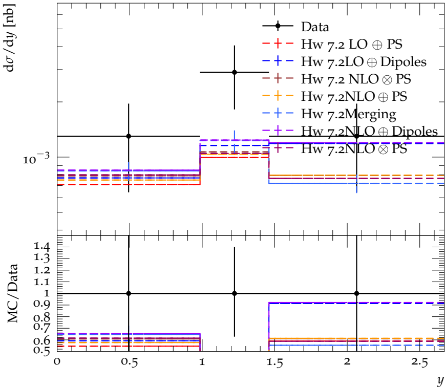
Rapidity w.r.t to sphericity axis for \Xi^- , \Xi^+ at 34.8 GeV
