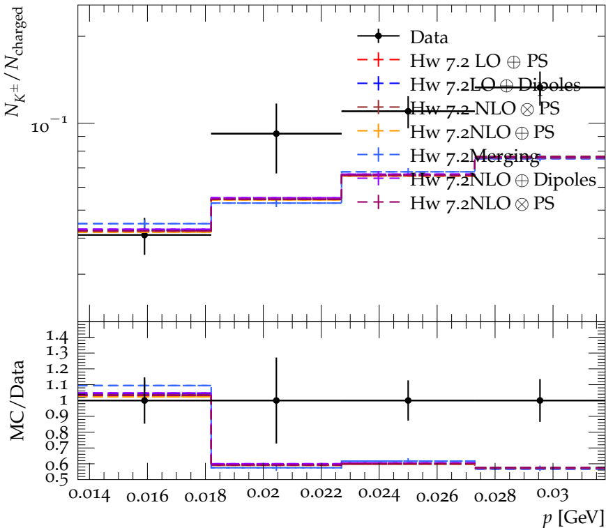
Ratio of K^\pm to charged particles at 44 GeV
