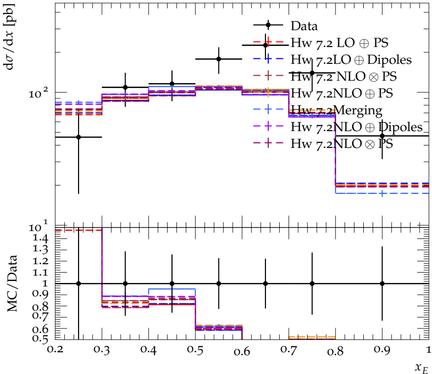
D^{*\pm} scaled energy spectrum (measured using D^0 \rightarrow K^- \pi^+ )
