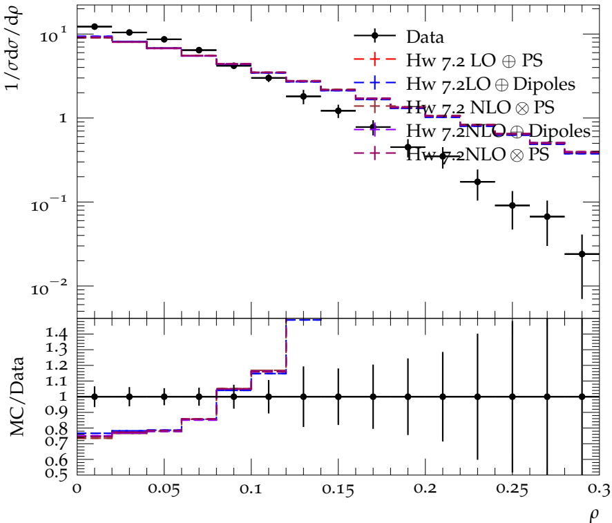
Scaled jet mass difference at 14 GeV
