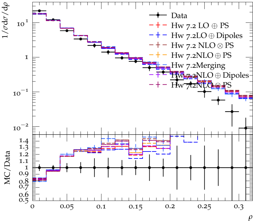
Scaled jet mass difference at 43.5 GeV
