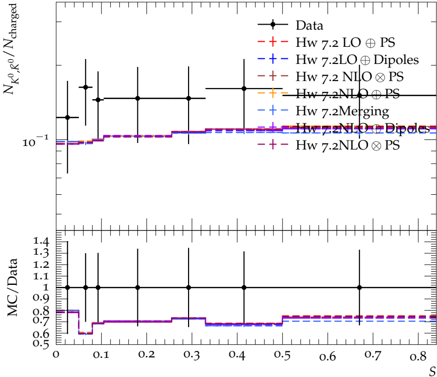
N_{K^0, \bar{K}^0} / N_{\text{charged}} vs sphericity at 21.5 GeV
