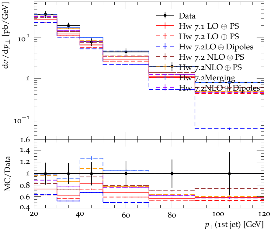
p_{\perp} of 1st jet (electron channel)
