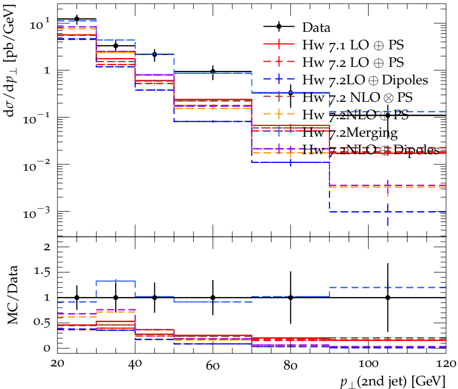
p_{\perp} of 2nd jet (electron channel)
