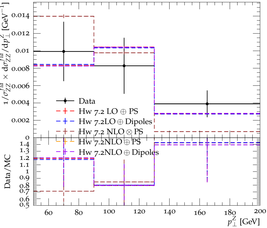
Differential cross-section for ZZ \rightarrow ll\nu\nu vs. p_{\perp}^Z
