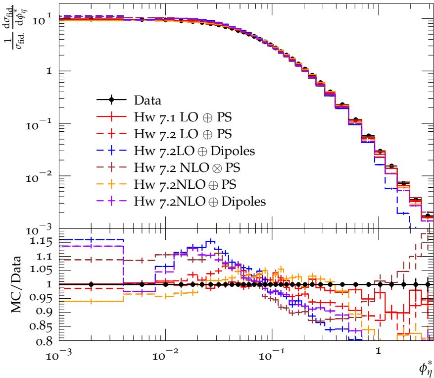
\phi_\eta^* spectrum, Z \rightarrow ee (bare)
