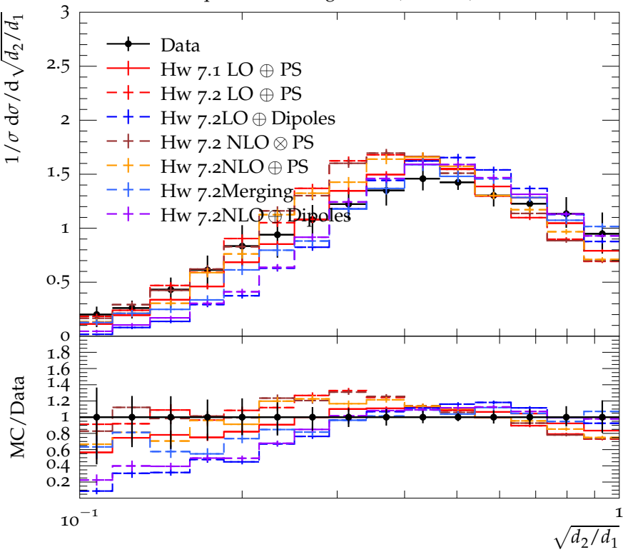
Ratio of subsequent clustering scales ( W \rightarrow e\nu )
