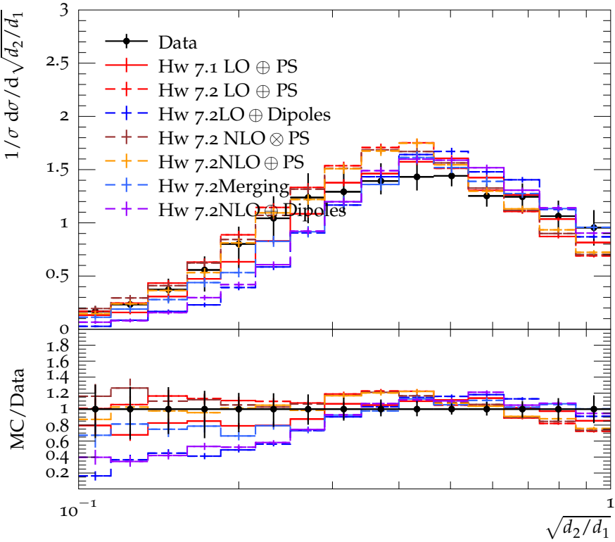
Ratio of subsequent clustering scales ( W \rightarrow \mu\nu )
