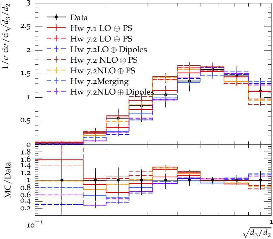
Ratio of subsequent clustering scales ( W \rightarrow e\nu )
