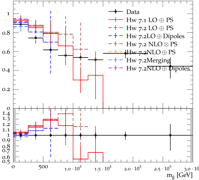
Jet veto efficiency vs. m_{jj} in the baseline region
