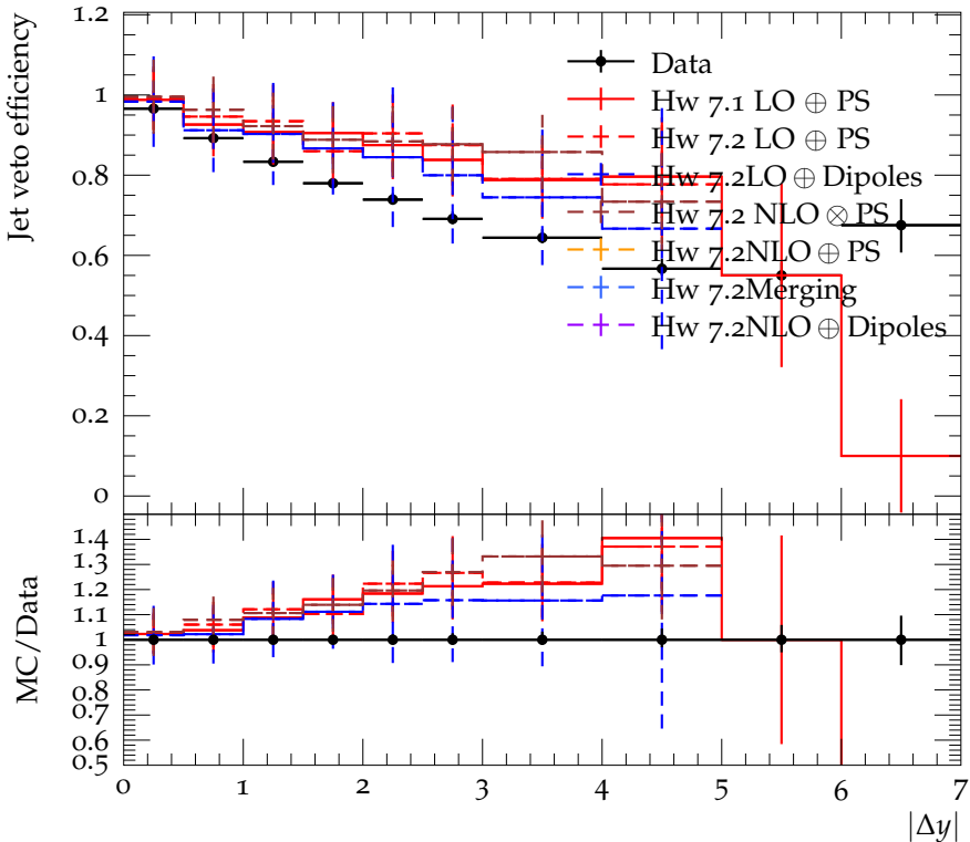
Jet veto efficiency vs. |\Delta y| in the baseline region
