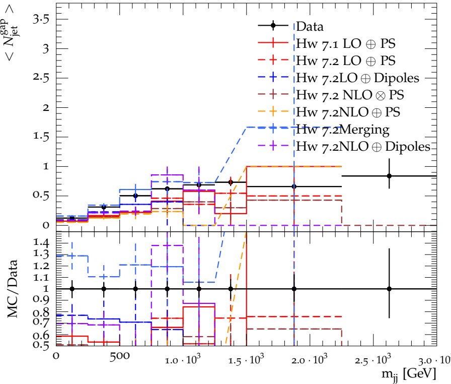
\langle N_{\text{jet}}^{\text{gap}} \rangle vs. m_{jj} in the baseline region
