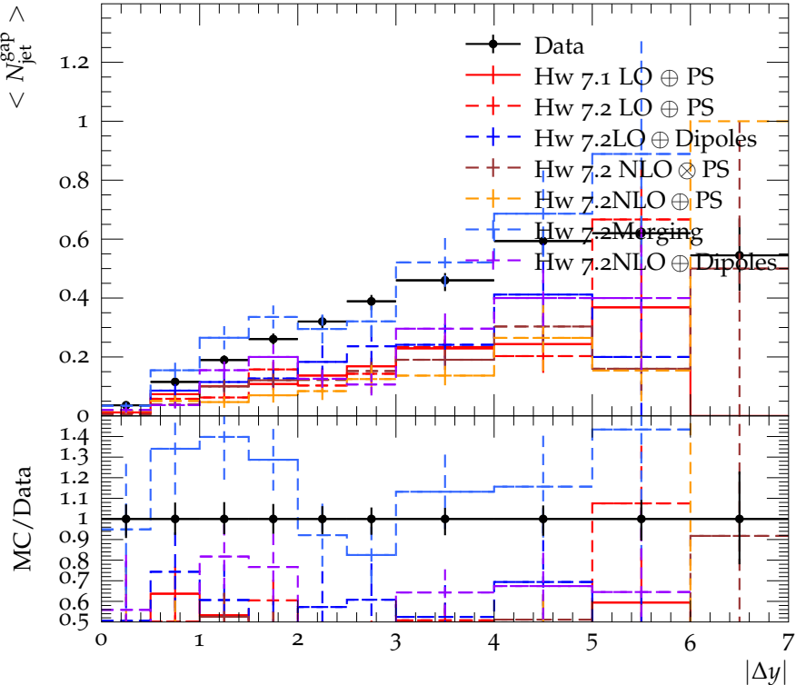
\langle N_{\text{jet}}^{\text{gap}} \rangle vs. |\Delta y| in the baseline region
