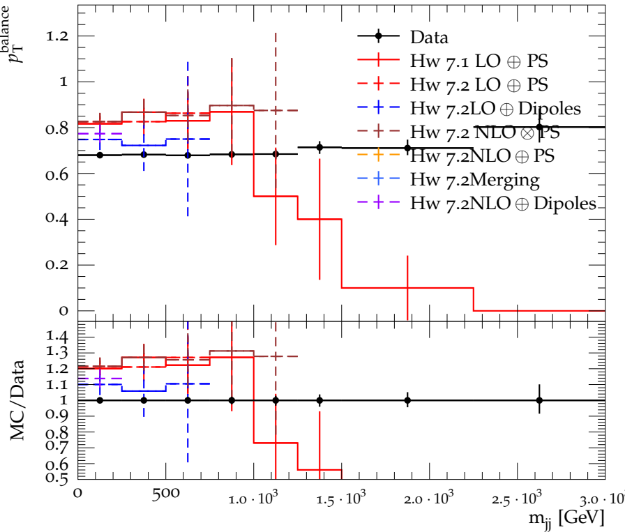
p_T^{\text{balance}} cut efficiency vs. m_{jj} in the baseline region
