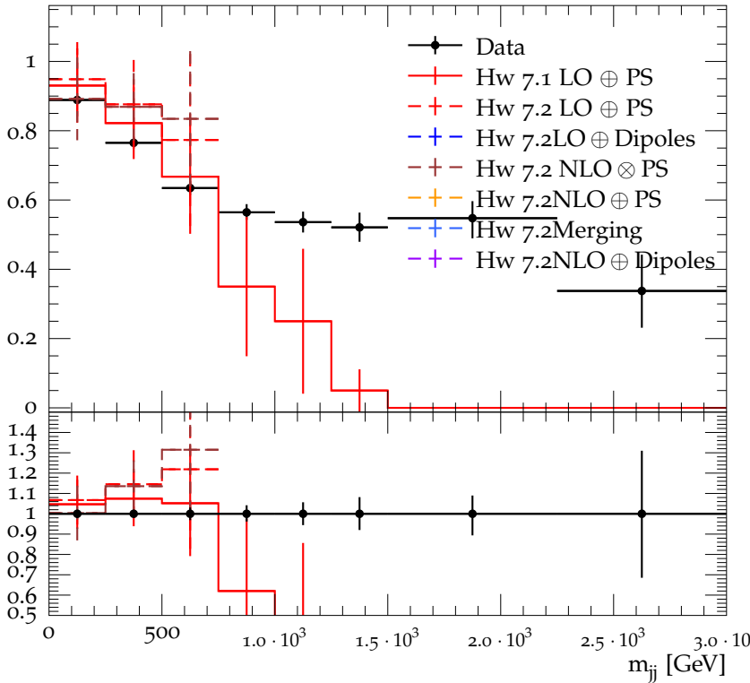
Jet veto efficiency vs. m_{jj} in the high- p_T region
