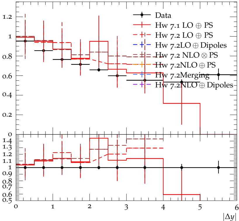
Jet veto efficiency vs. |\Delta y| in the high- p_T region
