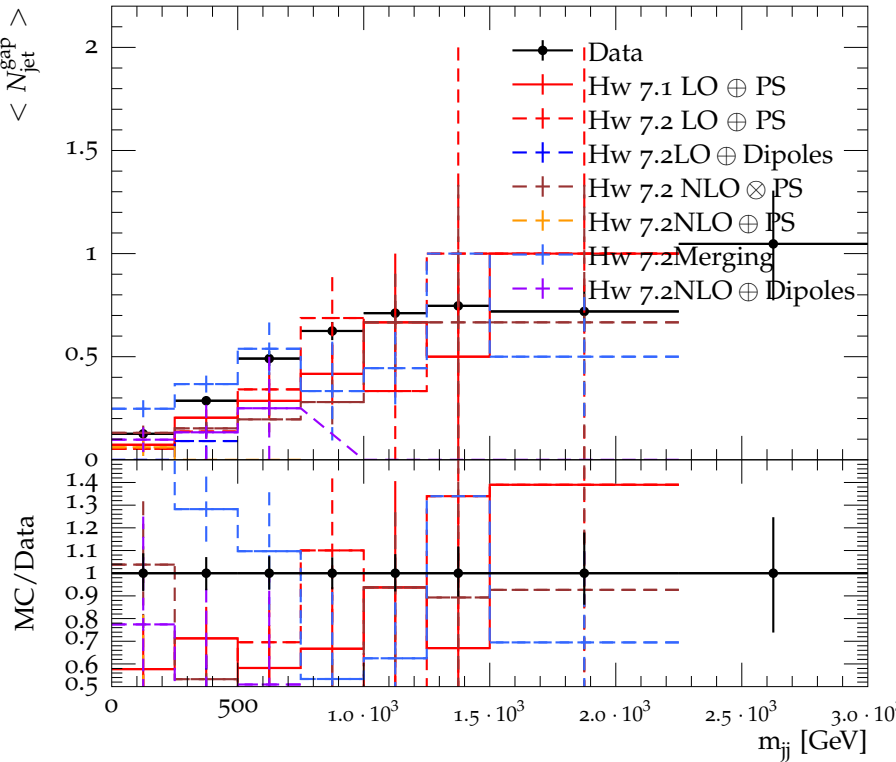
\langle N_{\text{jet}}^{\text{gap}} \rangle vs. m_{jj} in the high- p_T region
