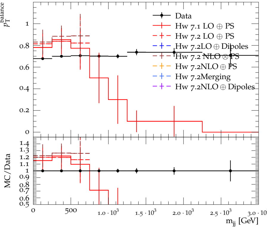
p_T^{\text{balance}} cut efficiency vs. m_{jj} in the high- p_T region
