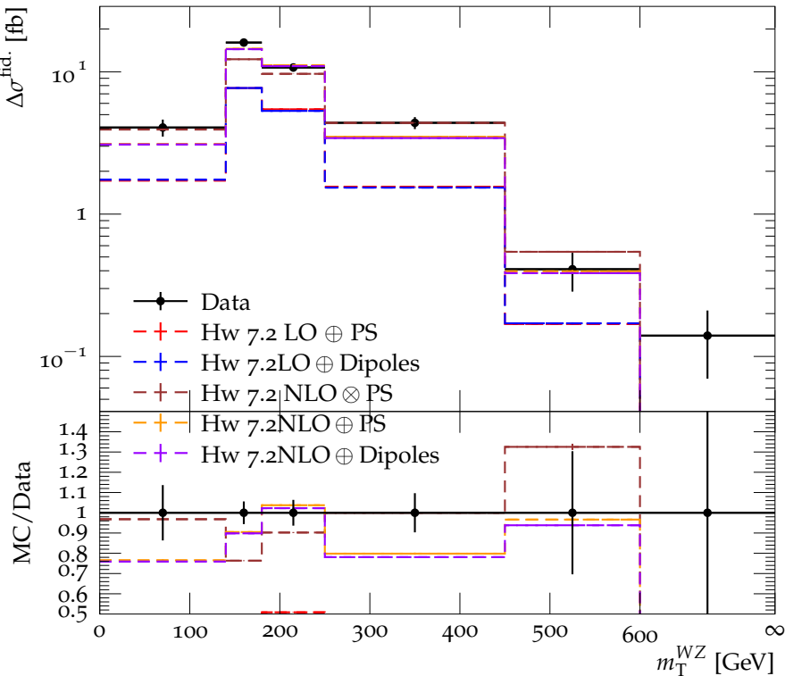
Differential fiducial W^\pm Z cross section as a function of m_T^{WZ}
