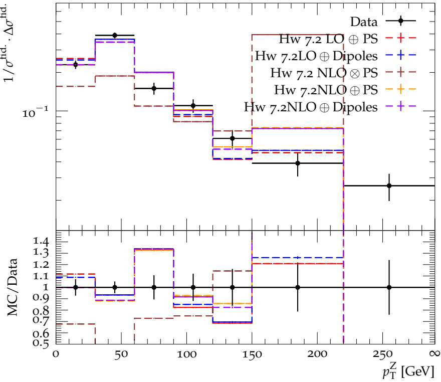
Normalised differential W^+Z cross section as a function of p_T^Z
