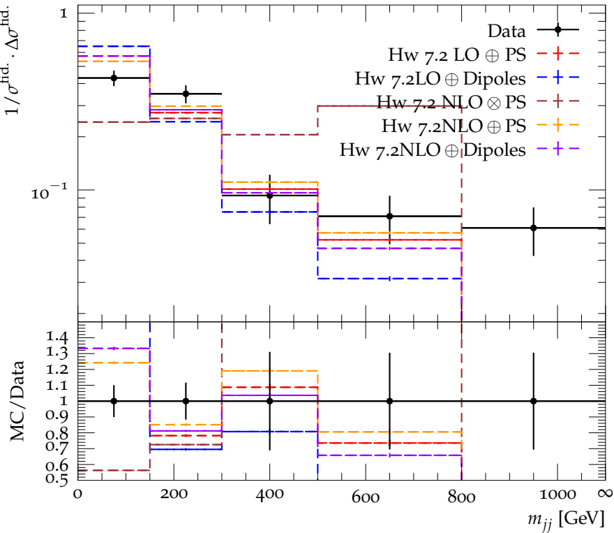
Normalised differential W^\pm Z cross section as a function of m_{jj}
