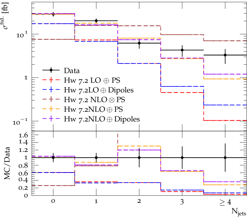
W^{\pm}Z \rightarrow \ell\nu\ell\ell fid. cross section as a function of the jet multiplicity
