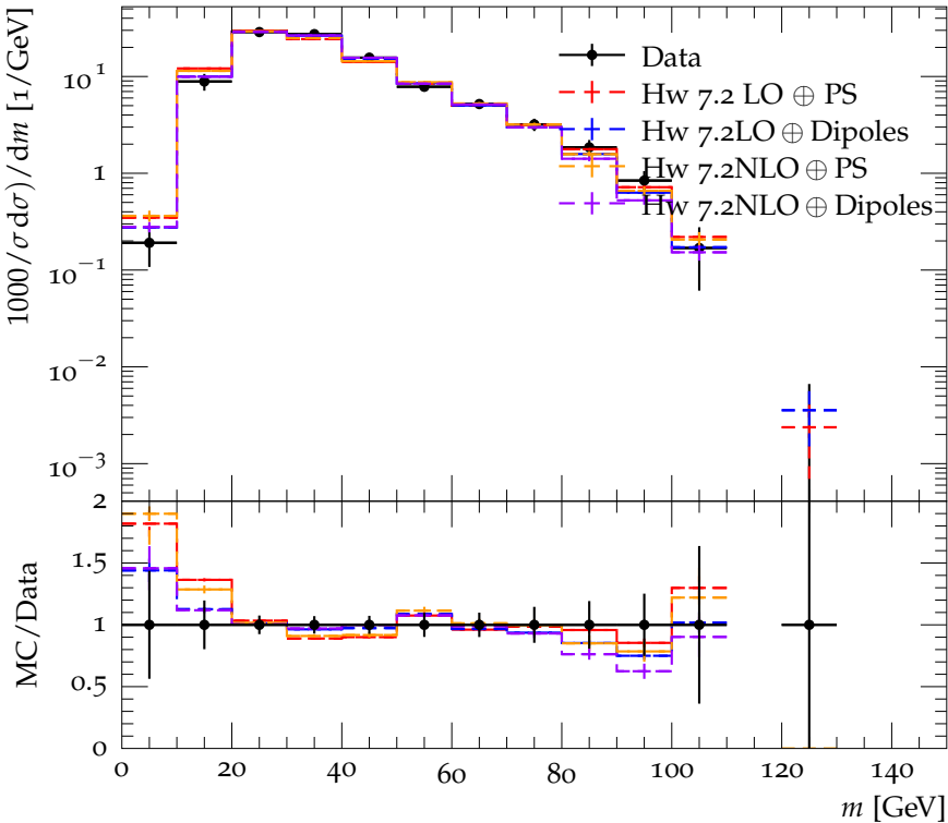
Filtered AK7 W+jets, p_{T,j} = 220-300 GeV
