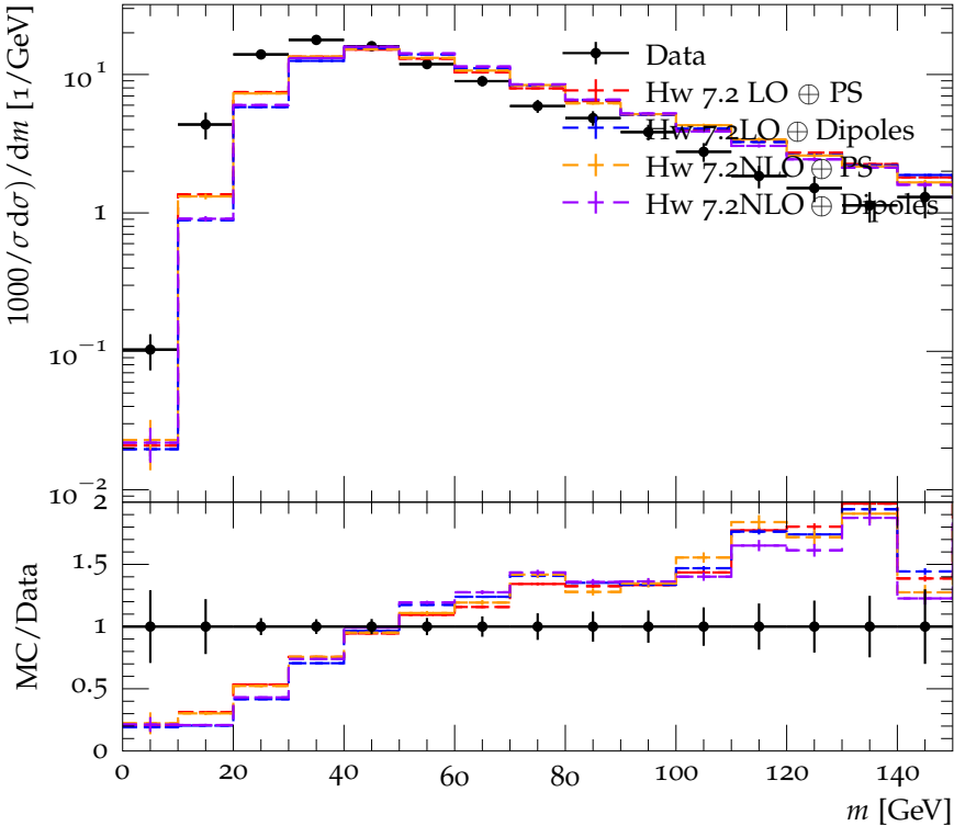
Filtered CA12 W+jets, p_{T,j} = 300\text{--}450 GeV
