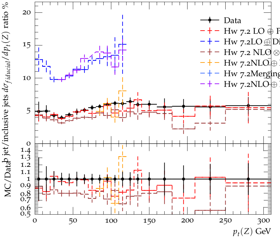
CMS, 8 TeV, Z boson p_t ratio, at least one b jet over inclusive
