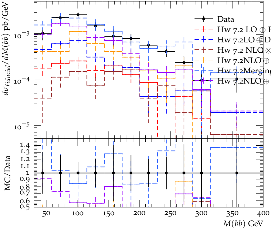
CMS, 8 TeV, bb system mass, at least two b jets
