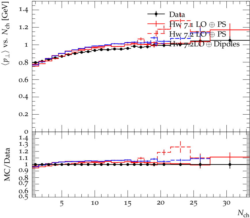
Avg. transv. momentum vs. N_{\text{ch}} ( 0.5 \leq p_{\perp} \leq 4 GeV)
